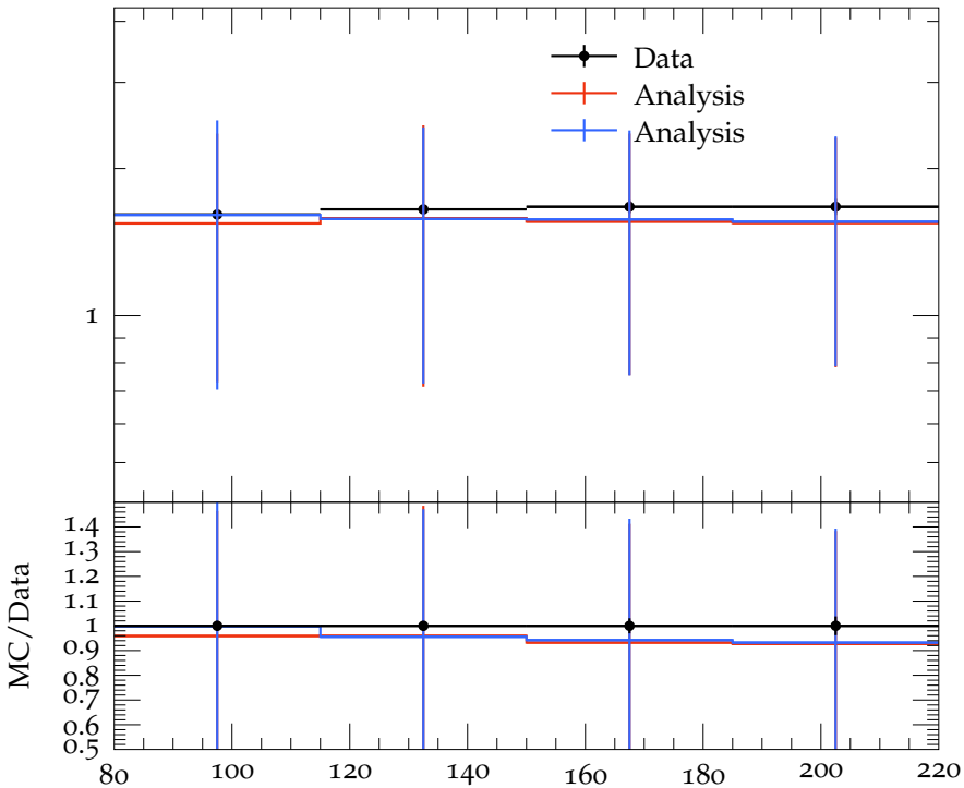
C_2 vs W , 2 < \eta < 3
