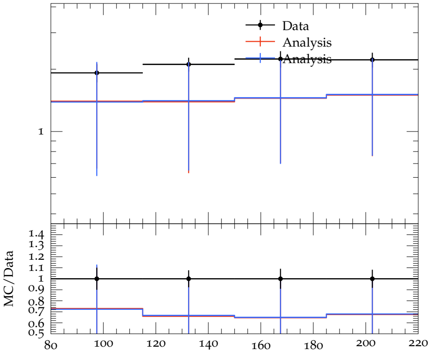
D_2 vs W , 2 < \eta < 3
