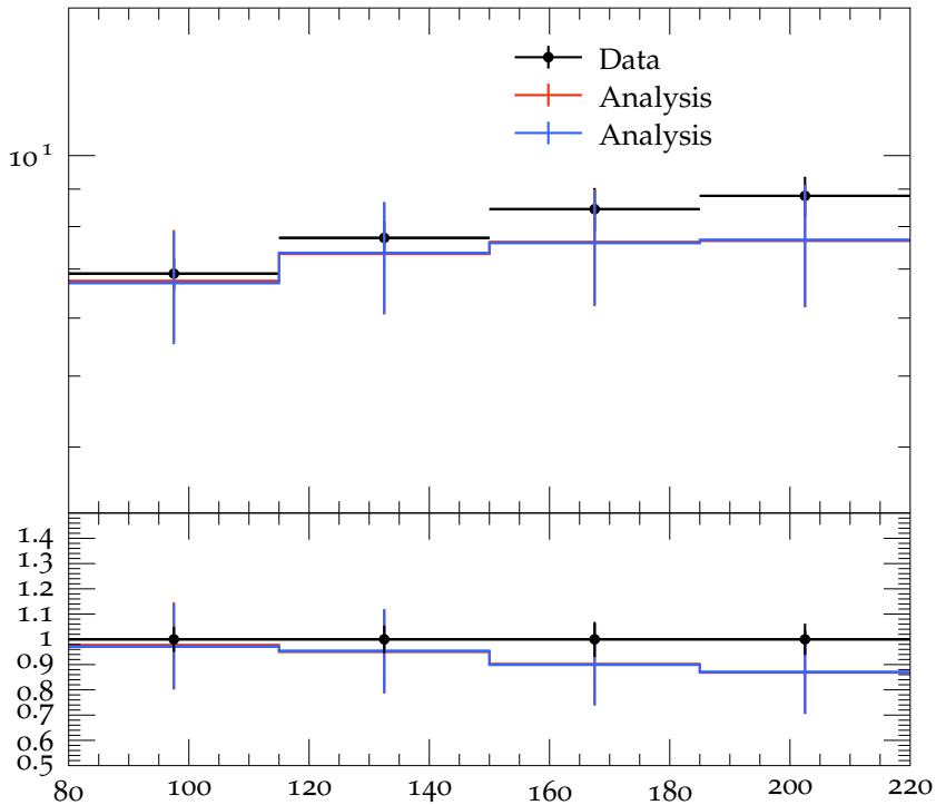
Mean multiplicity vs W , 1 < \eta < 5
