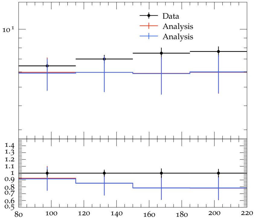
Mean multiplicity vs W , 1 < \eta < 4
