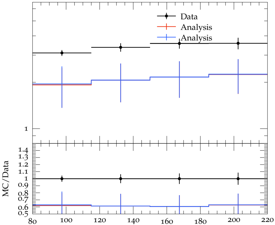
D_2 vs W , 1 < \eta < 3
