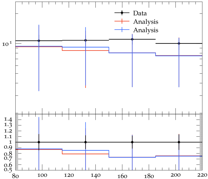
C_4 vs W , 1 < \eta < 2
