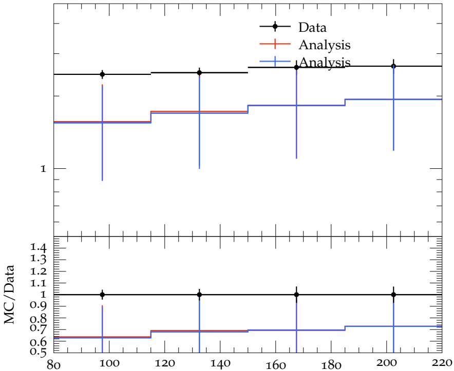
Mean multiplicity vs W , 1 < \eta < 2
