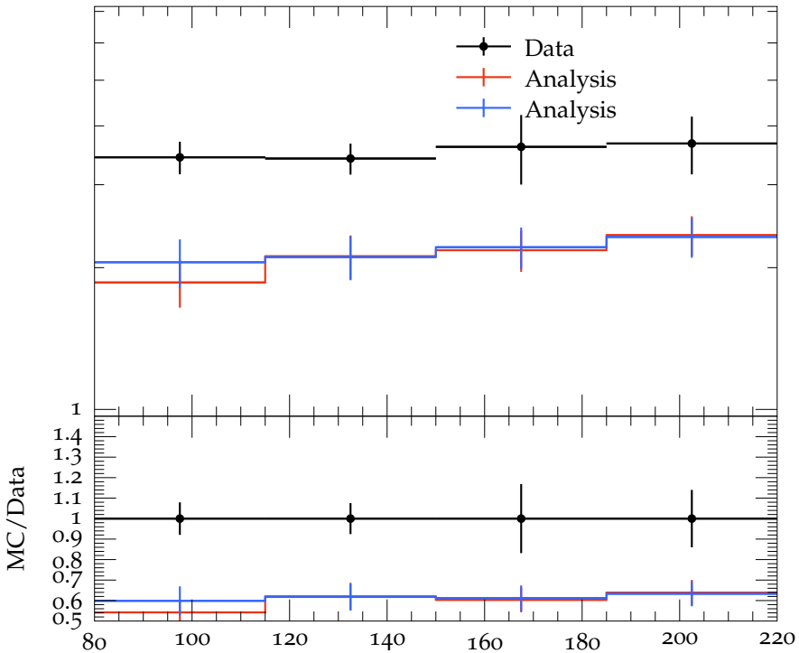
D_3 vs W , 0 < \eta
