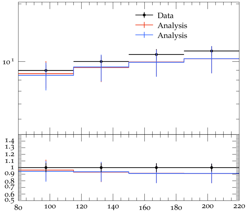
Mean multiplicity vs W , 0 < \eta
