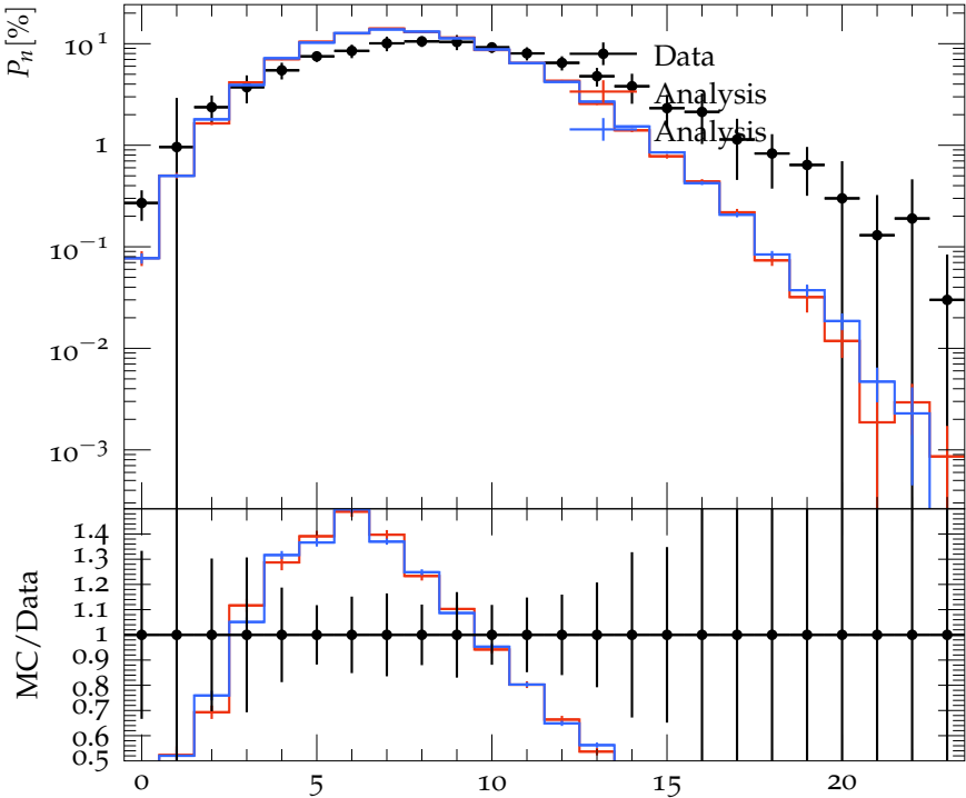
P_n vs multiplicity 1 < \eta < 5 , 185 < W < 220 GeV
