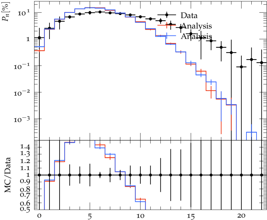
P_n vs multiplicity 1 < \eta < 4, 150 < W < 185 GeV
