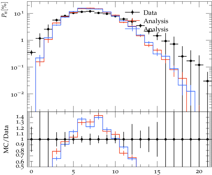
P_n vs multiplicity 1 < \eta < 5 , 115 < W < 150 GeV
