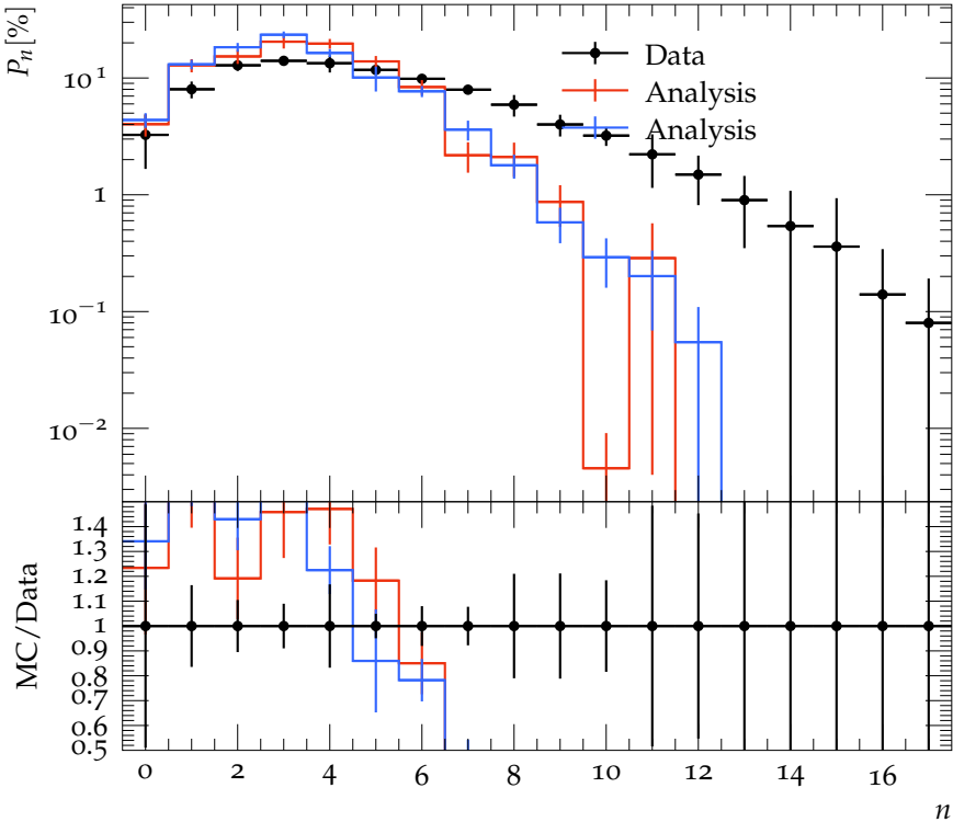
P_n vs multiplicity 1 < \eta < 3, 80 < W < 115 GeV
