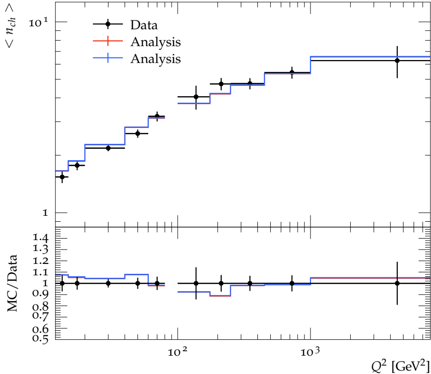
Average charged particle multiplicity vrs. Q^2
