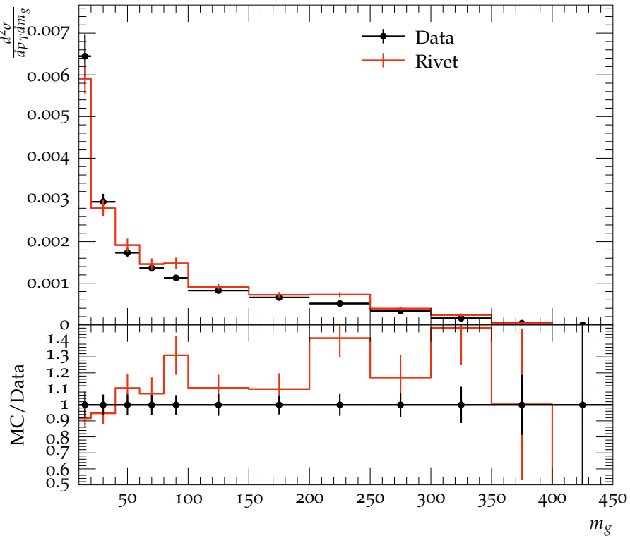
CMS, 13 TeV, Groomed jet mass m_g ( 760 < p_T < 900 GeV)
