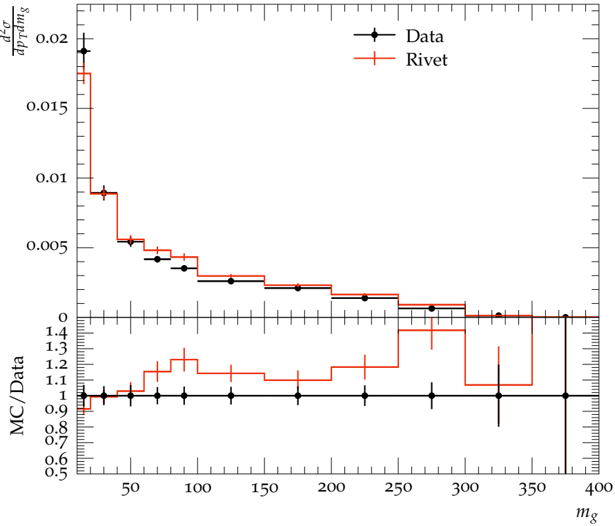
CMS, 13 TeV, Groomed jet mass m_g ( 650 < p_T < 760 GeV)
