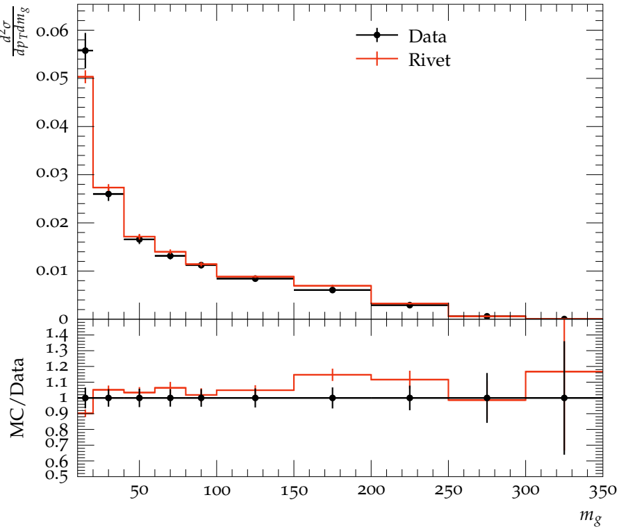
CMS, 13 TeV, Groomed jet mass m_g ( 550 < p_T < 650 GeV)
