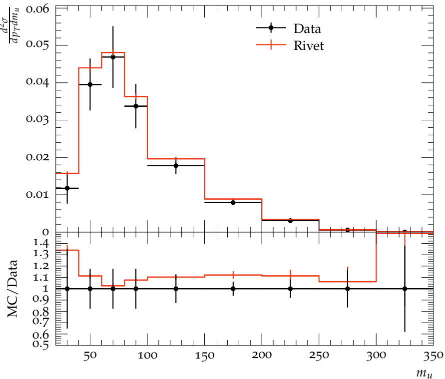
CMS, 13 TeV, Ungroomed jet mass m_u ( 550 < p_T < 650 GeV)
