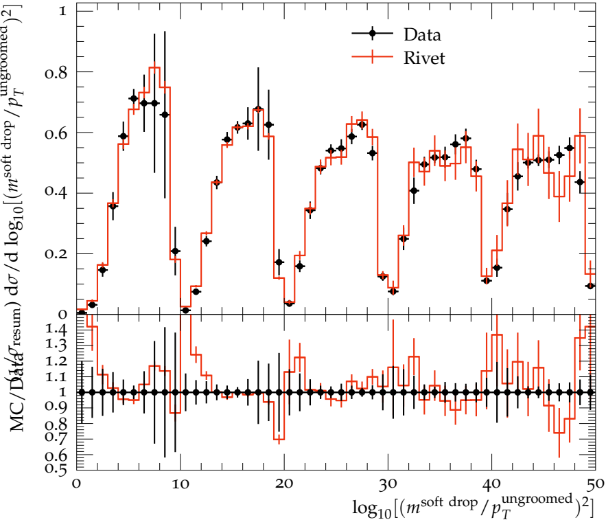
Dijet selection, Central jet, Cluster Based, Soft Drop \beta = 1.0 , z_{cut} =
