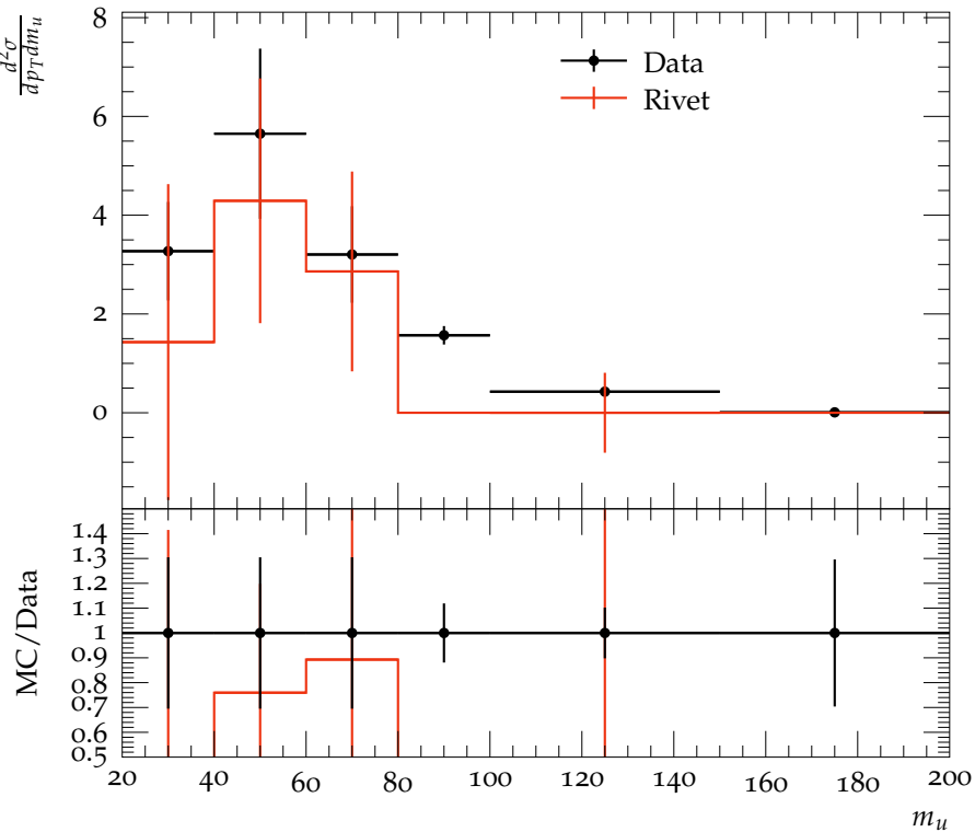
CMS, 13 TeV, Ungroomed jet mass m_u ( 260 < p_T < 350 GeV)
