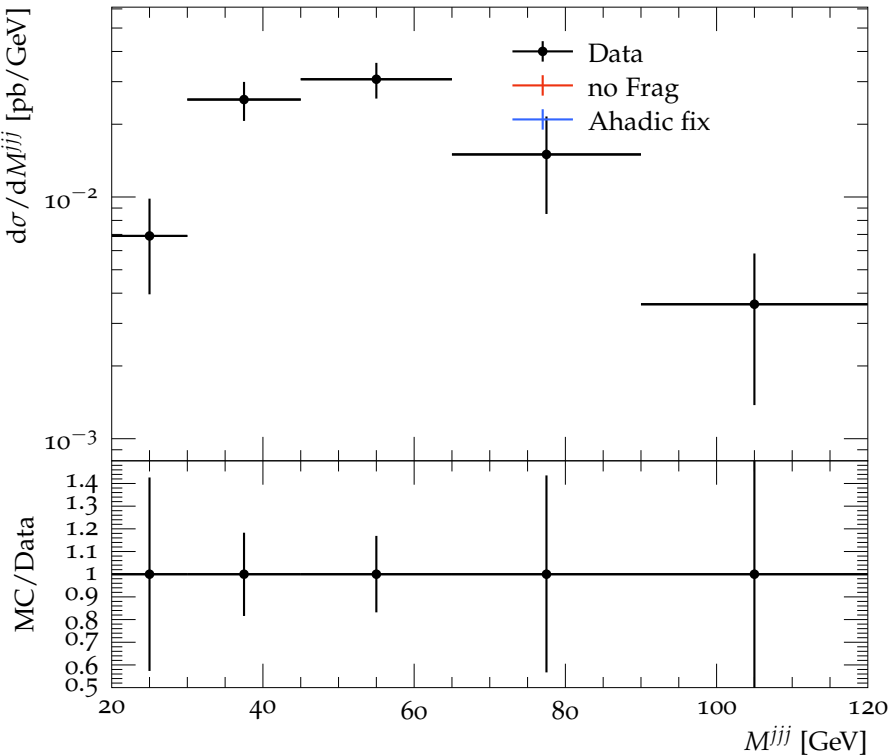
Unpolarized inclusive three jet cross section vs trijet mass.
