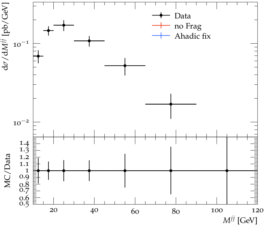
Unpolarized dijet cross section vs dijet mass.
