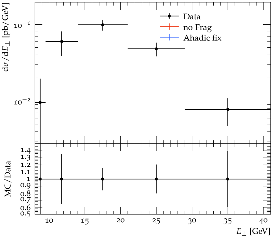
Unpolarized inclusive three jet cross section vs E_{\perp}, e^{-}
