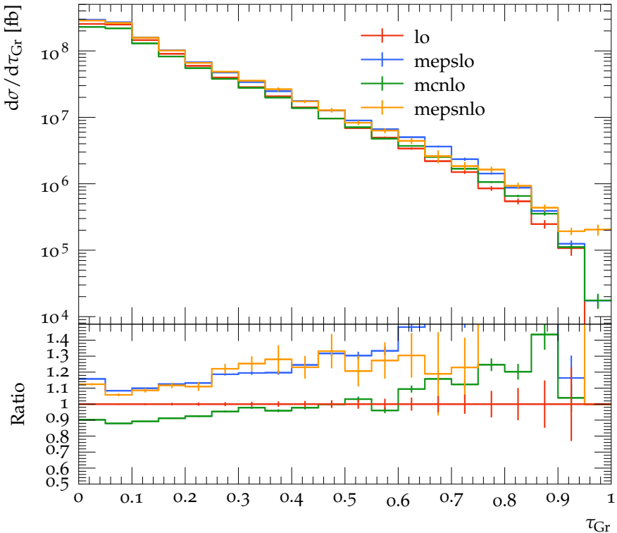
Groomed 1-jettiness \tau_{\text{Gr}} with z_{\text{cut}} = 0.5
