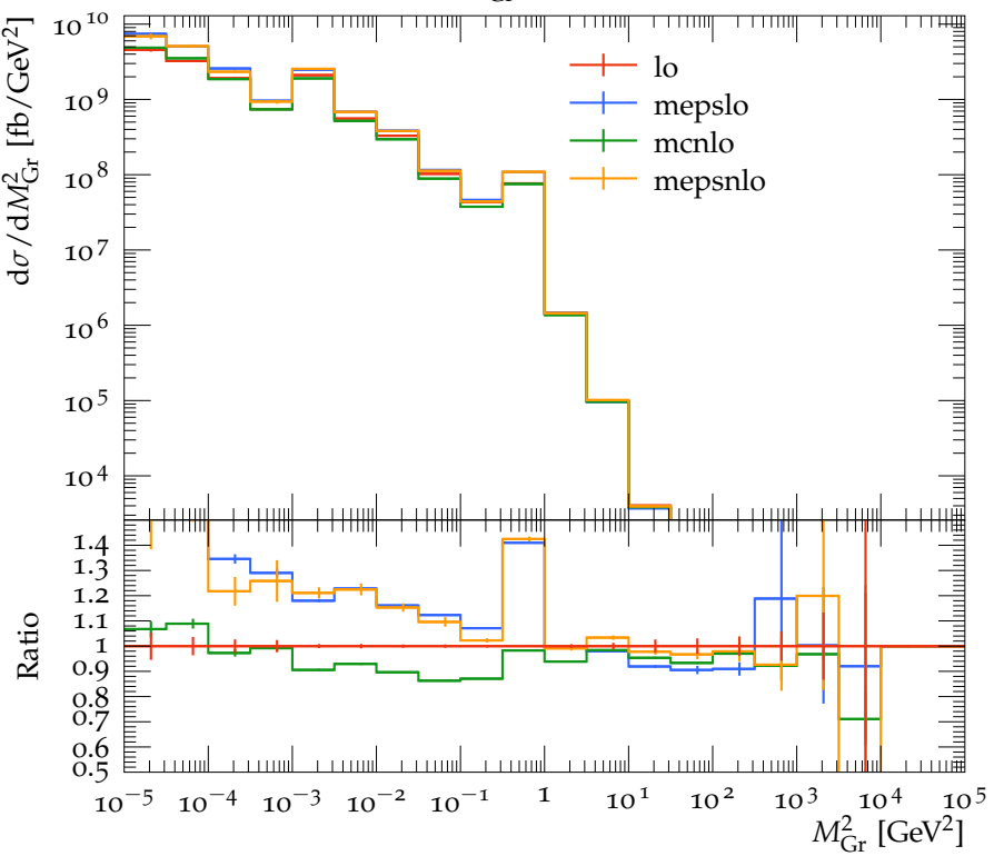
Groomed invariant mass M_{\text{Gr}}^2 with z_{\text{cut}} = 1
