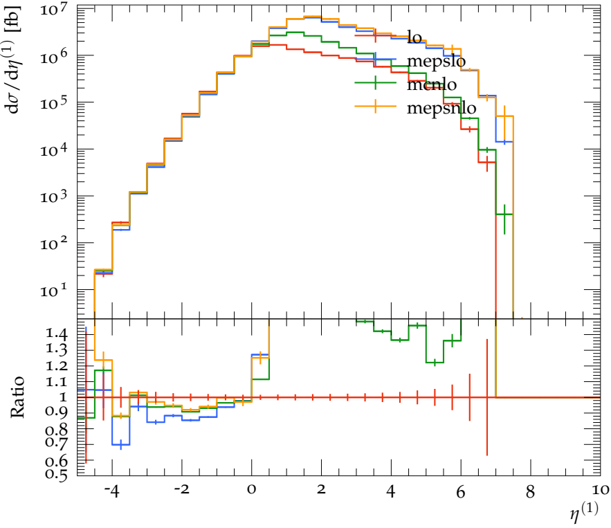
Leading jet pseudorapidity \eta
