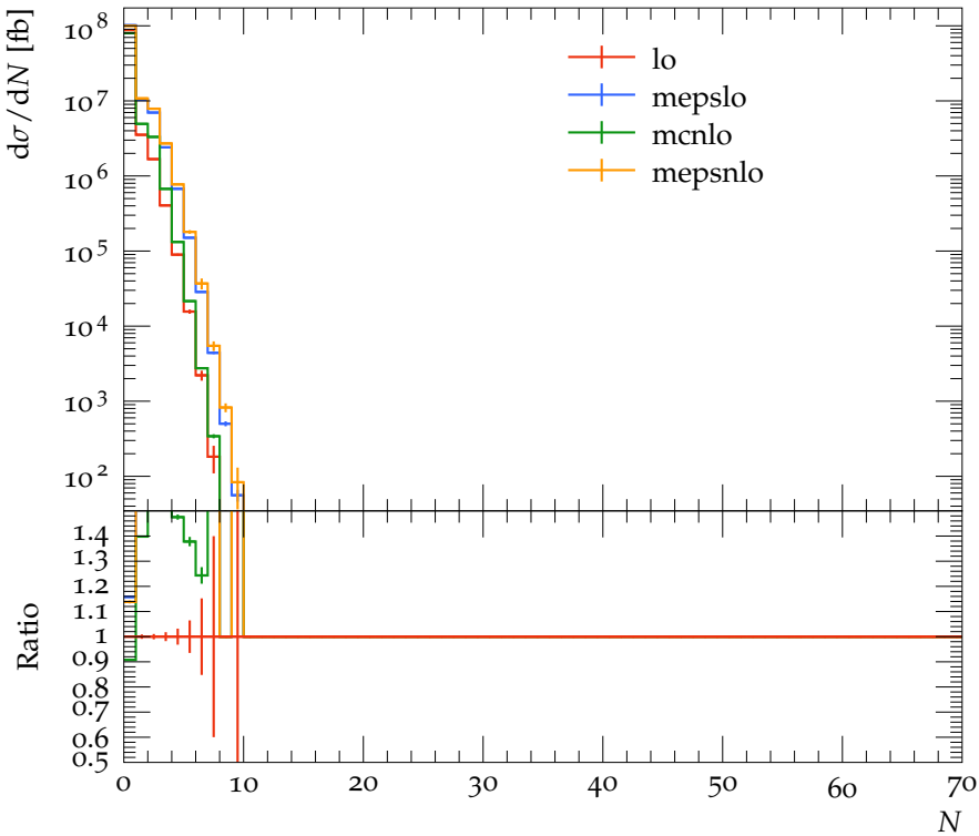
Jet multiplicity N
