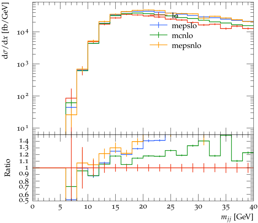
Distribution of dijet mass in bin of Q^2
