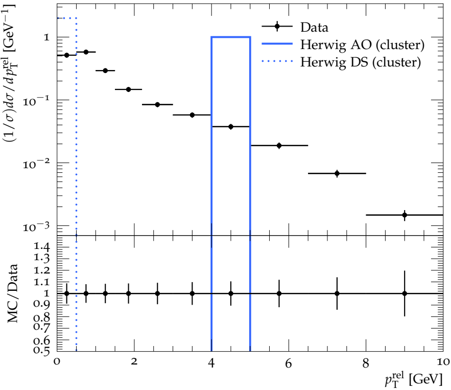
Transverse profile for 70 \text{ GeV} < p_T < 100 \text{ GeV}
