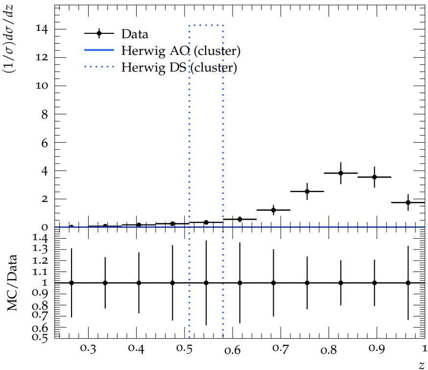
Longitudinal profile for 50 \text{ GeV} < p_T < 70 \text{ GeV}
