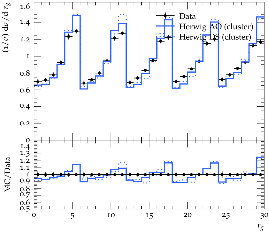
Dijet selection, Track Based, Soft Drop \beta = 0.0 , z_{cut} = 0.1
