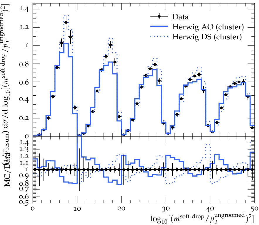
Dijet selection, Track Based, Soft Drop \beta = 2.0 , z_{cut} = 0.1
