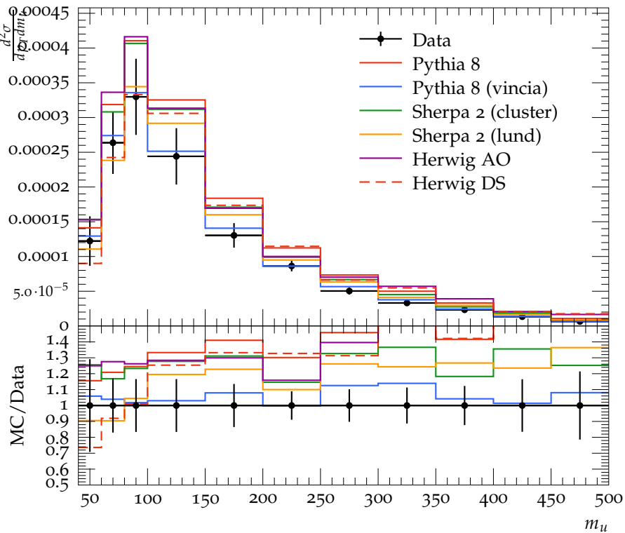
CMS, 13 TeV, Ungroomed jet mass m_u ( 1100 < p_T < 1200 GeV)
