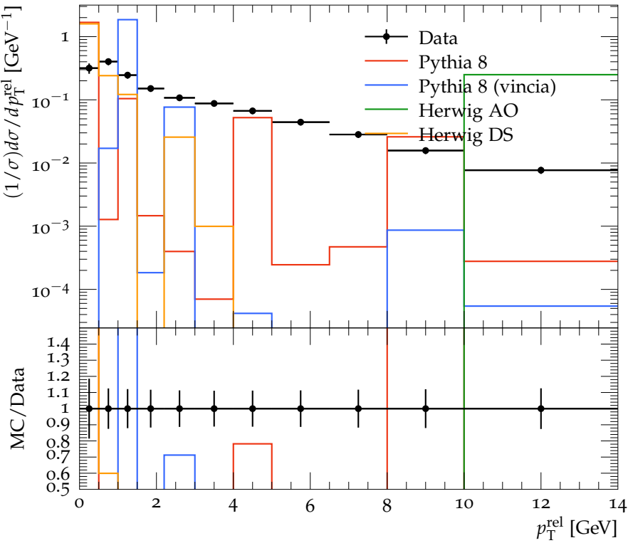
Transverse profile for p_T > 100 GeV
