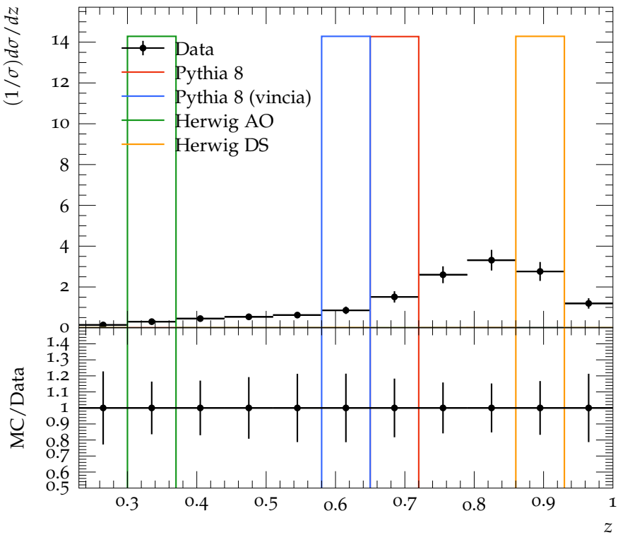
Longitudinal profile for 70 \text{ GeV} < p_T < 100 \text{ GeV}
