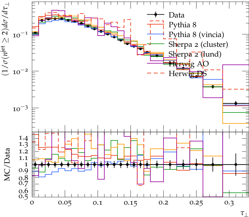
Transverse Thrust for n^{\text{jet}} = 5, H_{T2} > 2.0 \text{ TeV}
