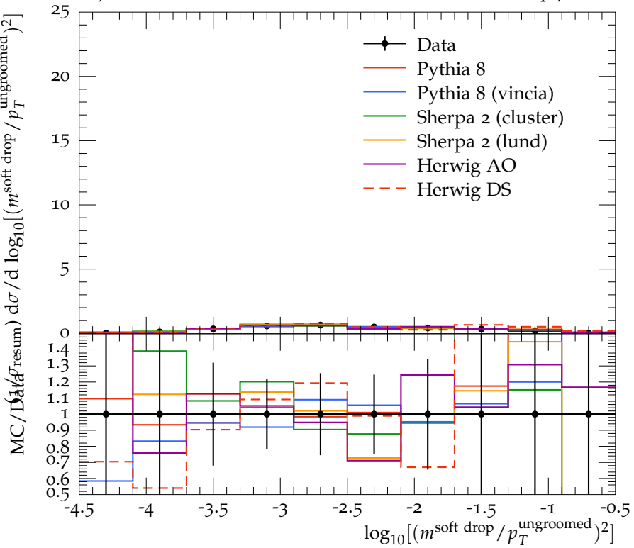
Dijet selection, Quark extraction, Track Based, Soft Drop \beta = 2.0 , z_{\text{cut}} = 0.1
