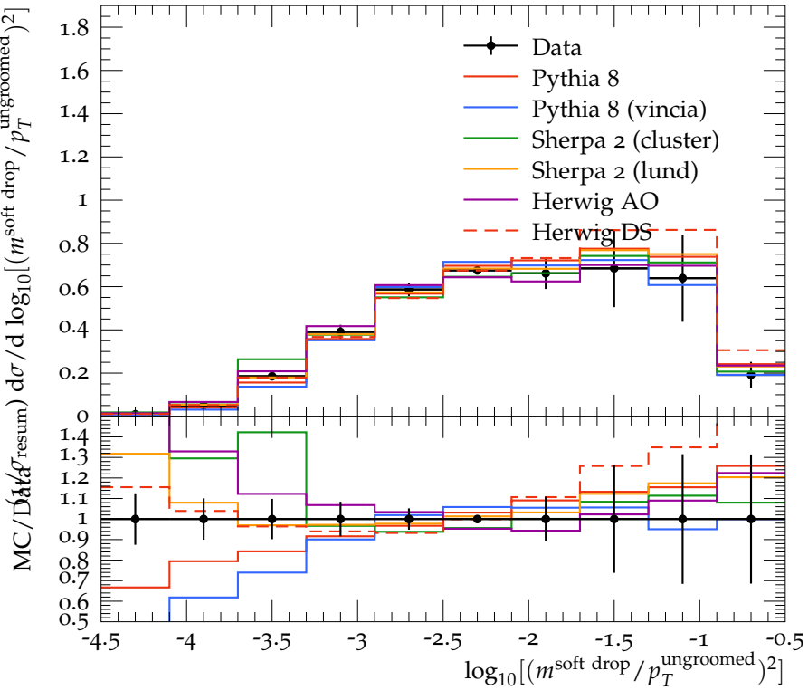
Dijet selection, Cluster Based, Soft Drop \beta = 1.0 , z_{cut} = 0.1
