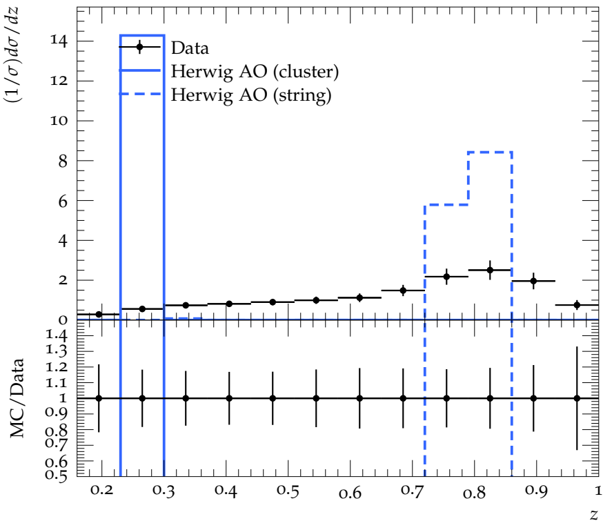
Longitudinal profile for p_T > 100 GeV
