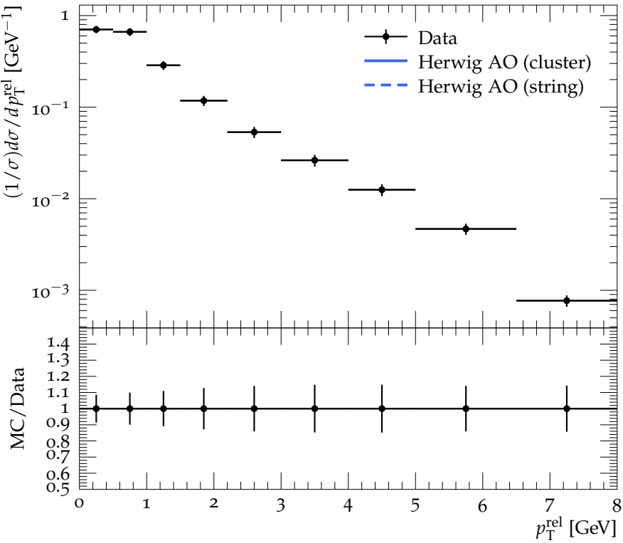
Transverse profile for 50 \text{ GeV} < p_T < 70 \text{ GeV}
