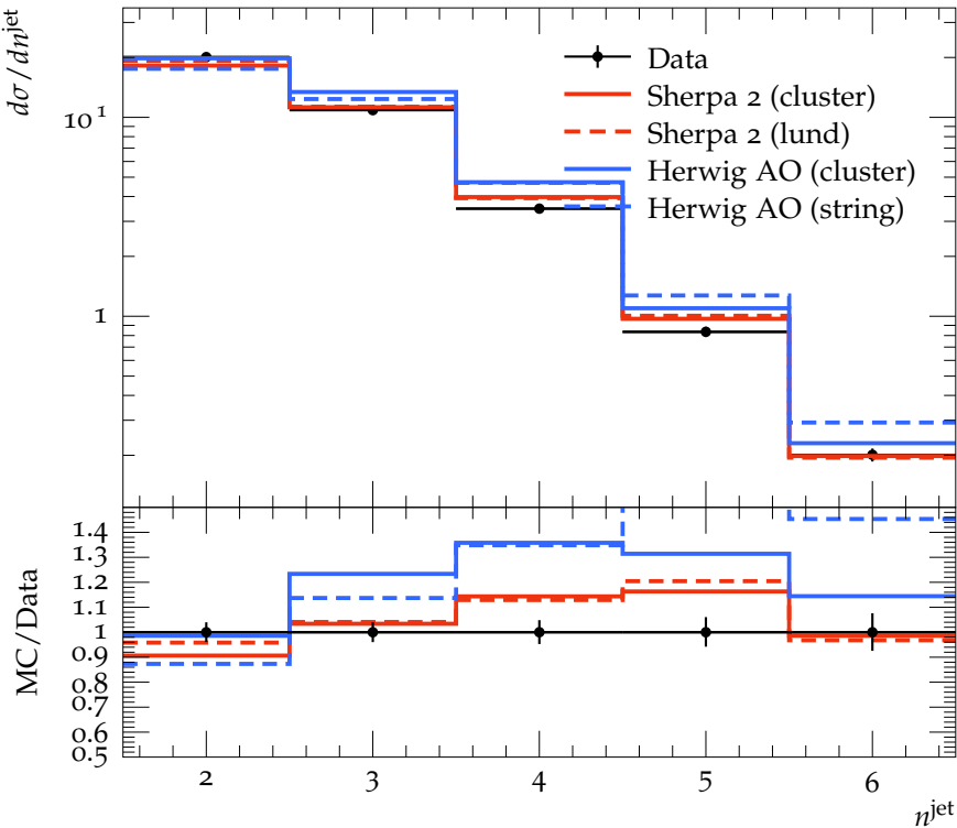
Jet multiplicity for 1.5 \text{ TeV} < H_{T2} < 2.0 \text{ TeV}
