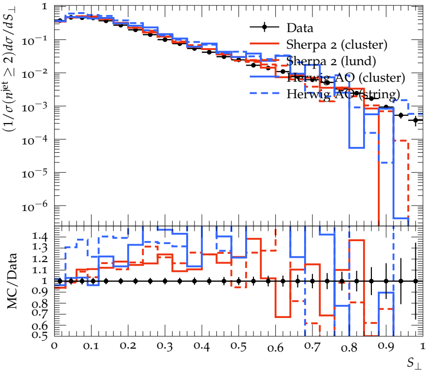
Transverse Sphericity for n^{\text{jet}} = 4 , H_{T2} > 2.0 TeV
