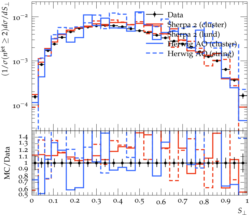
Transverse Sphericity for n^{\text{jet}} \geq 6 , 1.0 \text{ TeV} < H_{T2} < 1.5 \text{ TeV}
