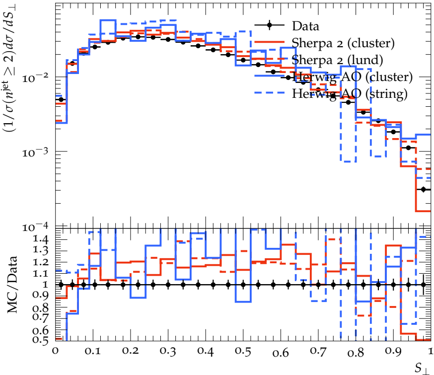
Transverse Sphericity for n^{\text{jet}} = 5 , 1.0 \text{ TeV} < H_{T2} < 1.5 \text{ TeV}
