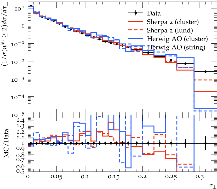
Transverse Thrust for n^{\text{jet}} = 3 , H_{T2} > 2.0 TeV
