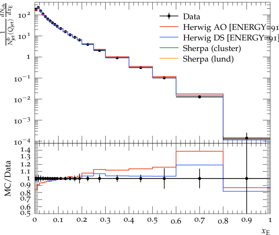
b hemisphere jet fragmentation, at 91.2 GeV
