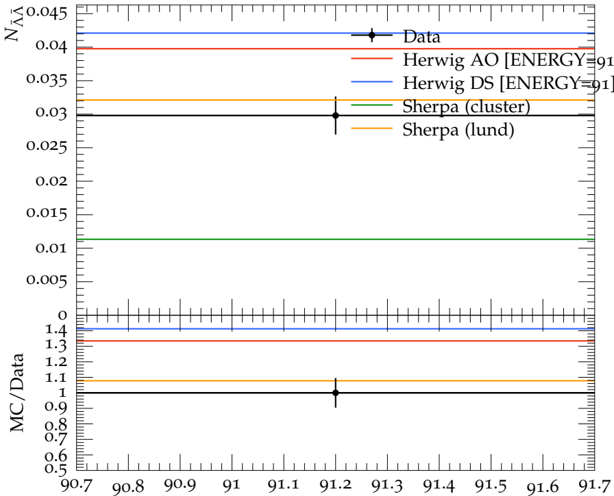
\Lambda\Lambda + \bar{\Lambda}\bar{\Lambda} pair multiplicity (3 jet events)
