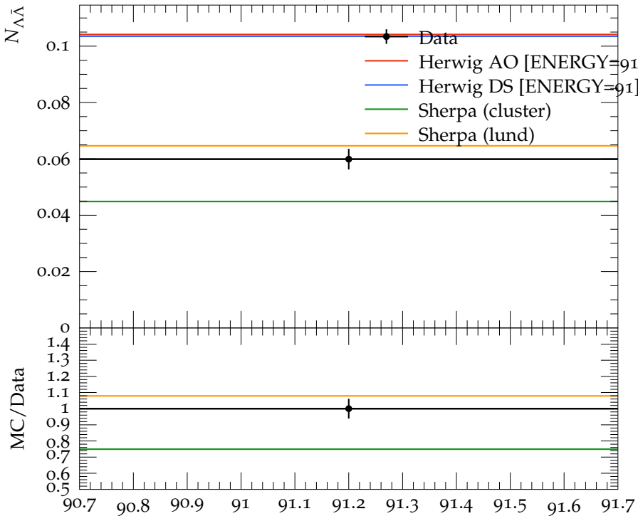
\Lambda\bar{\Lambda} pair multiplicity (2 jet events)
