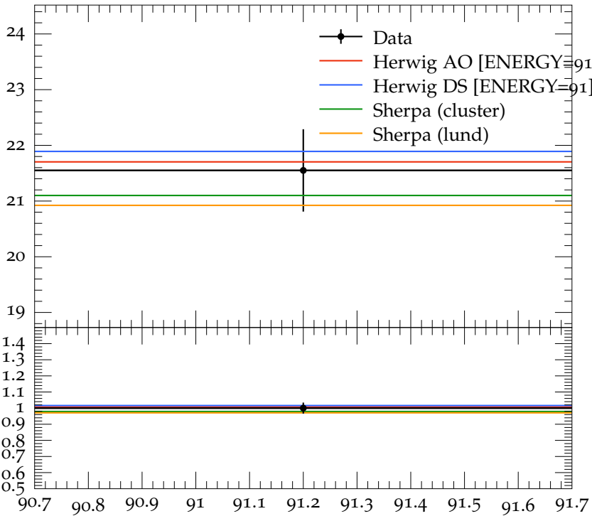
c events mean charged multiplicity
