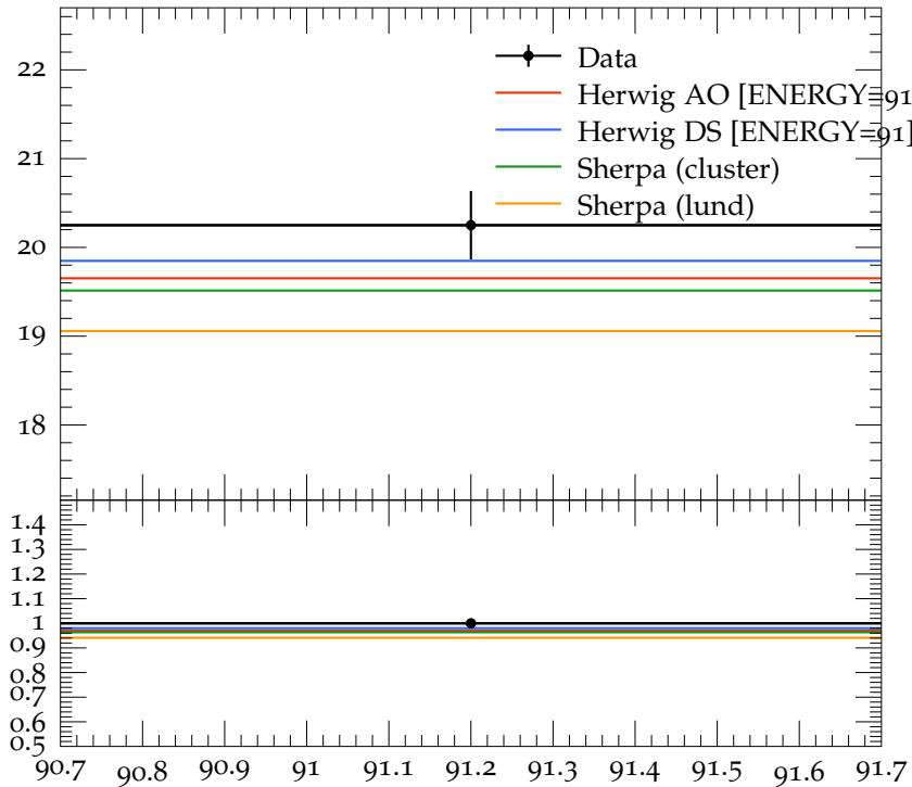
uds events mean charged multiplicity
